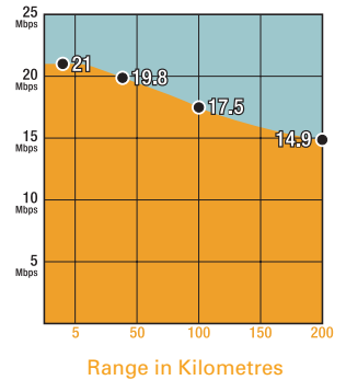
Performance with 5.8 and 5.4 GHz Connectorised Lite Models
