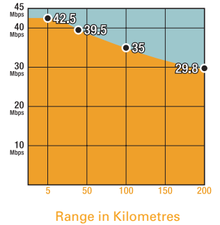
Performance with 5.8 and 5.4 GHz Connectorised Models
